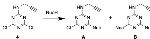
Scheme 2. Reaction of Alkyne Dichlorotriazine with Nucleophile
