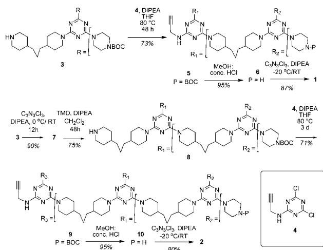
Scheme 1. Synthesis of Poly(dichlorotriazine) Dendrimers 1 and 2 a
