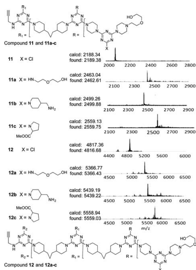
Figure 2. ESI mass spectrograms of dendrimer derivatives.
